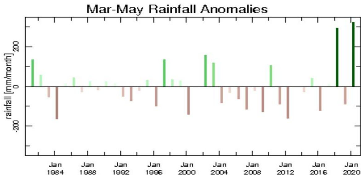
Figure 7: Time trend for MAM distribution of rainfall in time from 1980 – 2000
